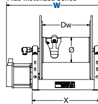
1125 Motorized Series
