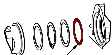
BEARING ASSY. DETAIL
